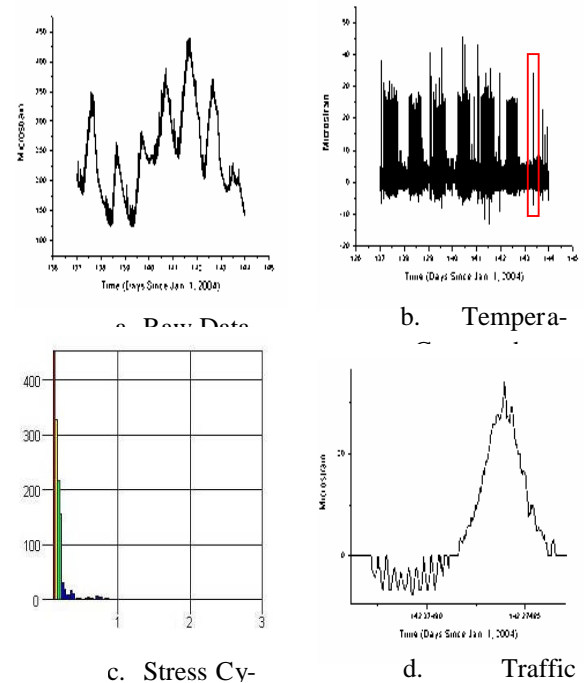
Figure 2. Typical strain data – bottom flange of girder
